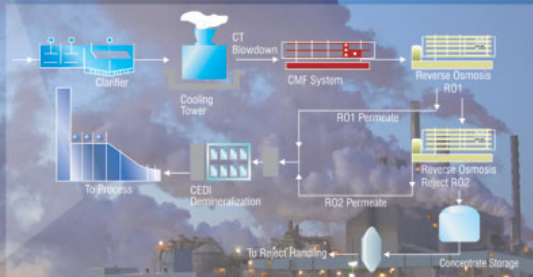
A typical integrated power plant ERS system
