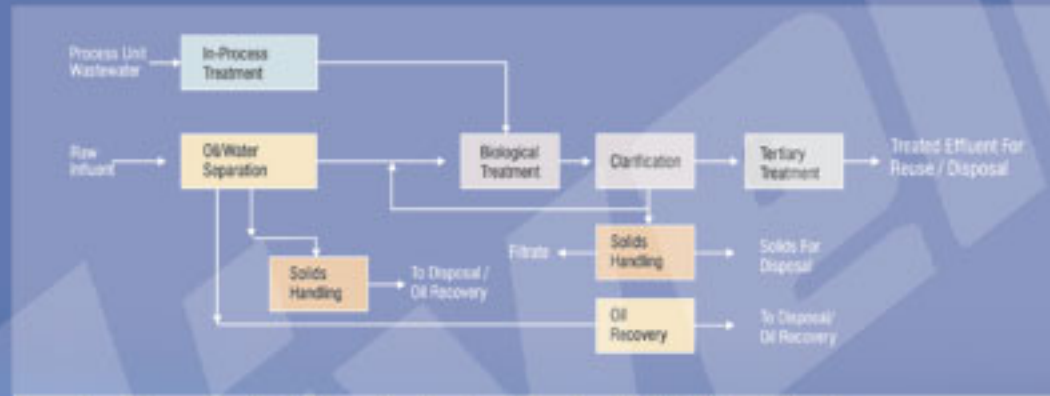
A typical wastewater treatment system for Petrochemical/ Oil & Gas industries
